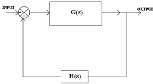
Fig. 9 Block Diagram in Simulink 7.0
