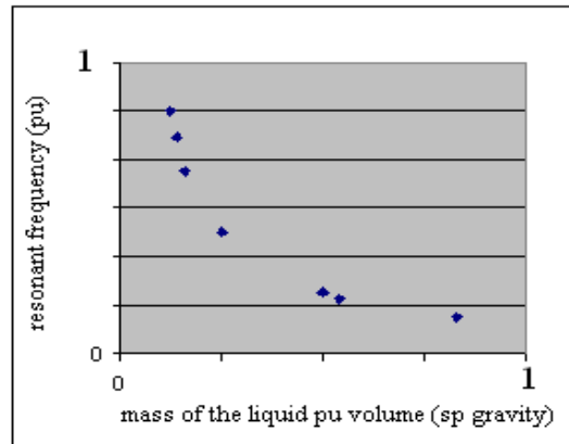
Fig. 7 Relation of Mass of the Liquid and Resonant Frequency
