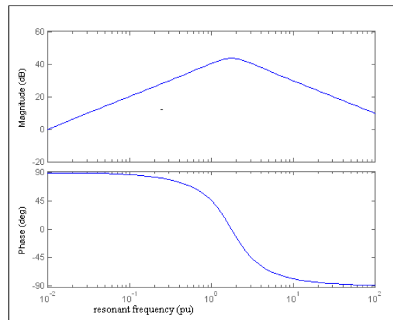
Fig. 4 Relation of Frequency Vs Gain
