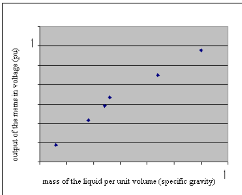
Fig. 5 Relation of Specific Gravity of Liquid and Output Voltage of MEMS
